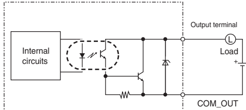
Output Circuit
